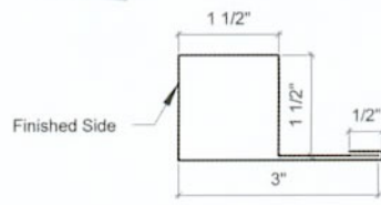
Snow Guard * Available Length: 10'
